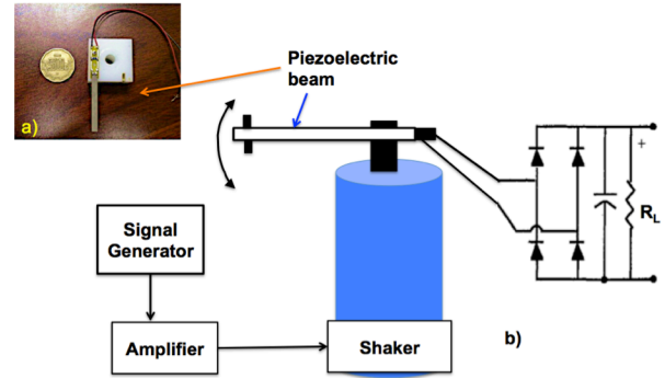
Fig. 2. (a) Piezoelectric cantilever as vibration transducer, (b) the experimental setup for the characterization of EH vibration source.
